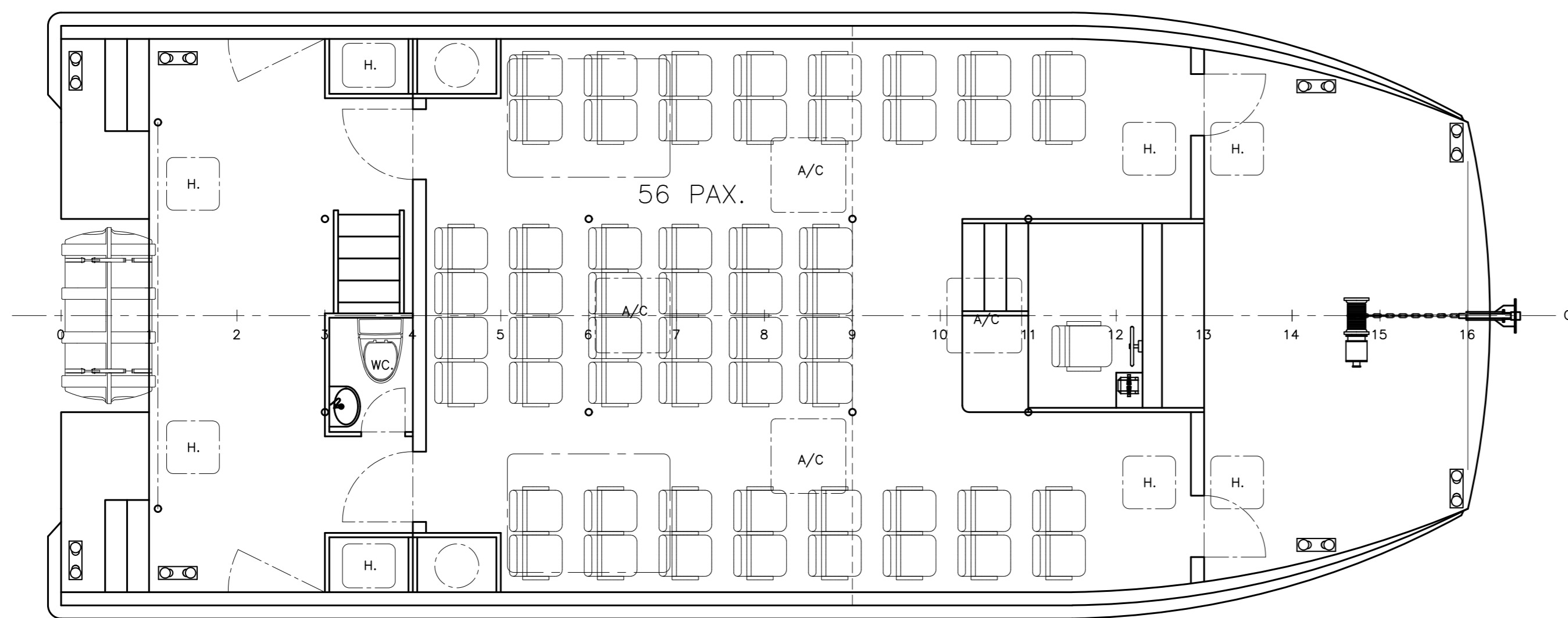
MAIN DECK PLAN SCALE 1:50
