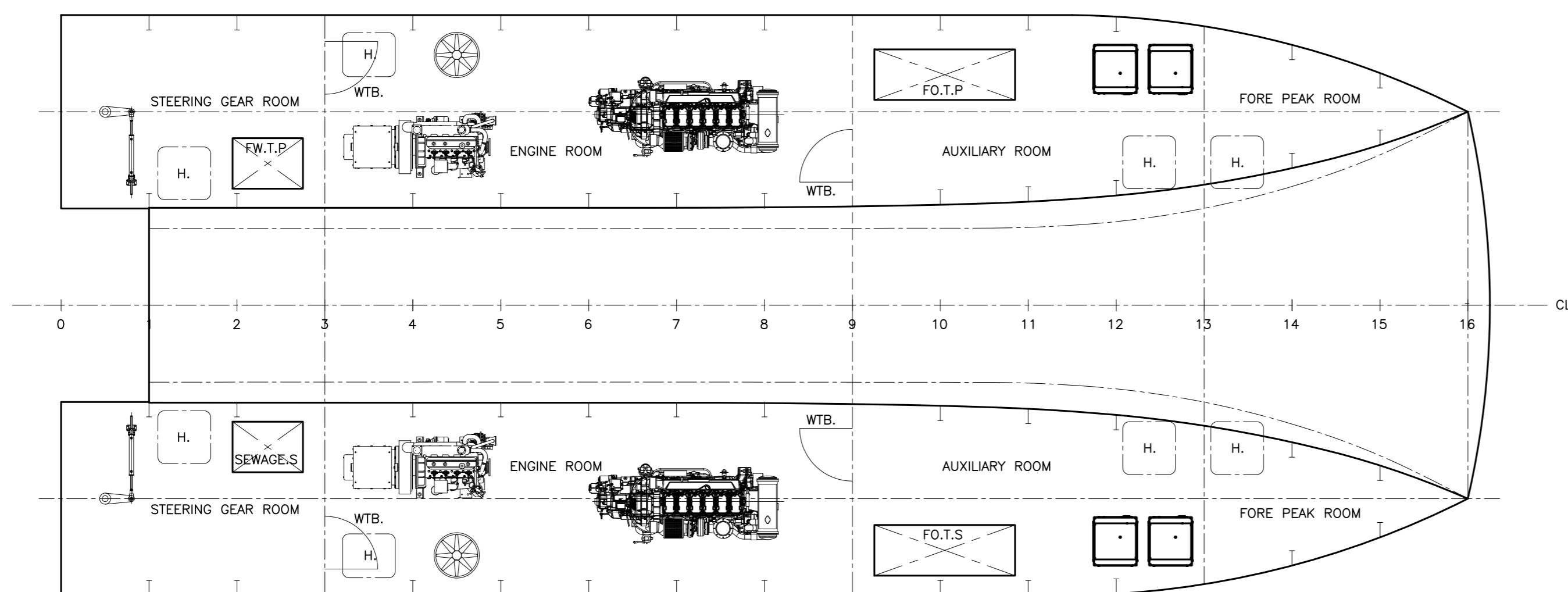
LOWER DECK PLAN SCALE 1:50
