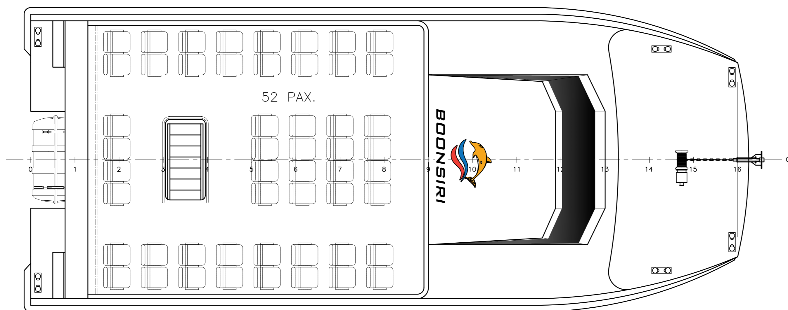
UPPER DECK PLAN SCALE 1:50
