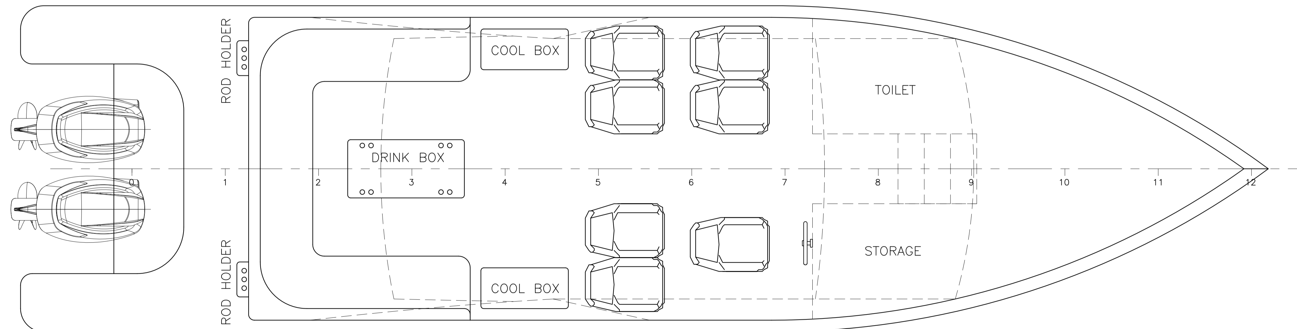
PLAN SCALE 1:20
