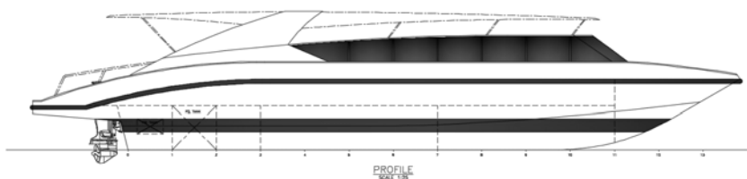
PROFILE SCALE 1:50
